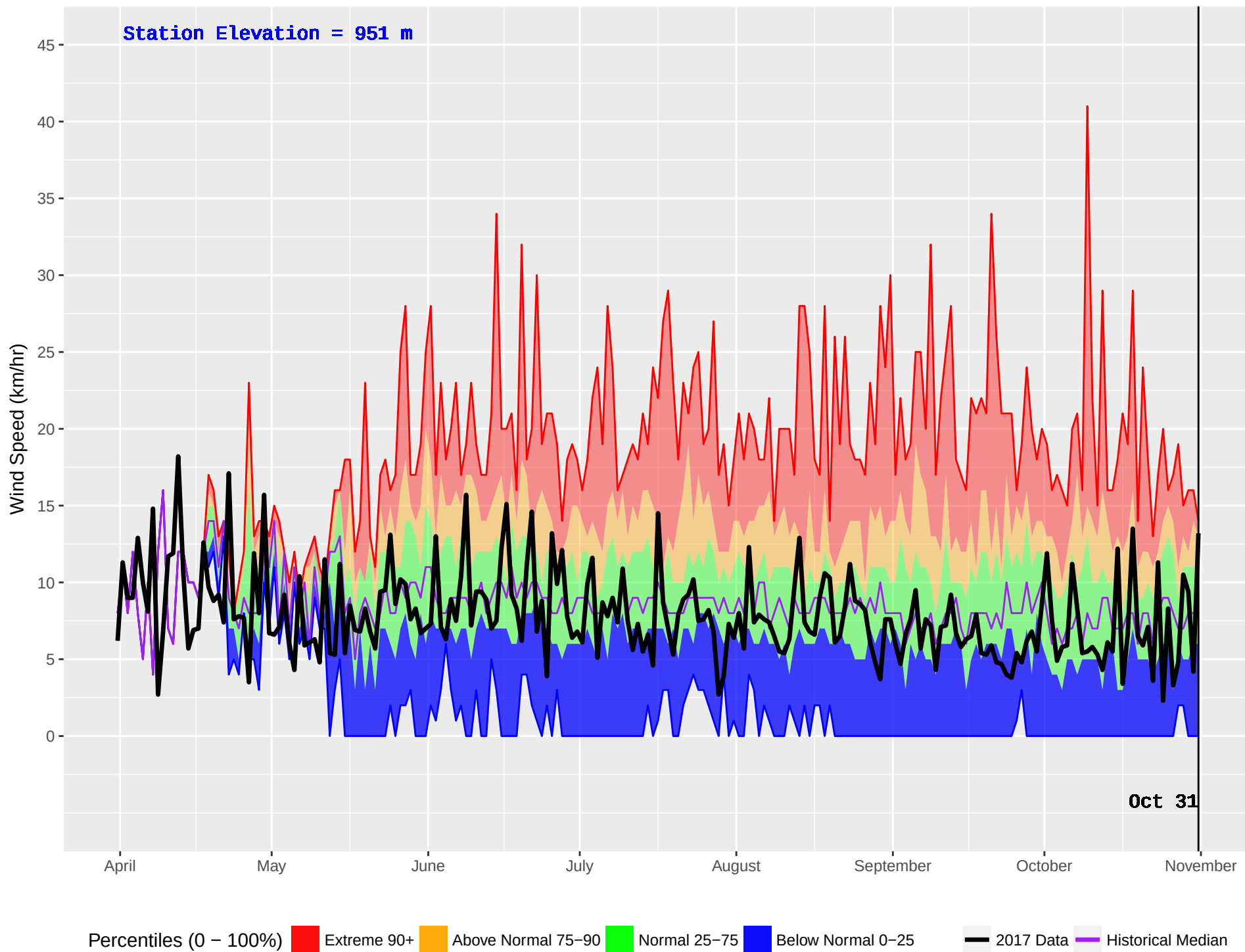
NORTH BABINE (173) : Historical (1986–2016) and Current (2017) Noon Wind Speed
