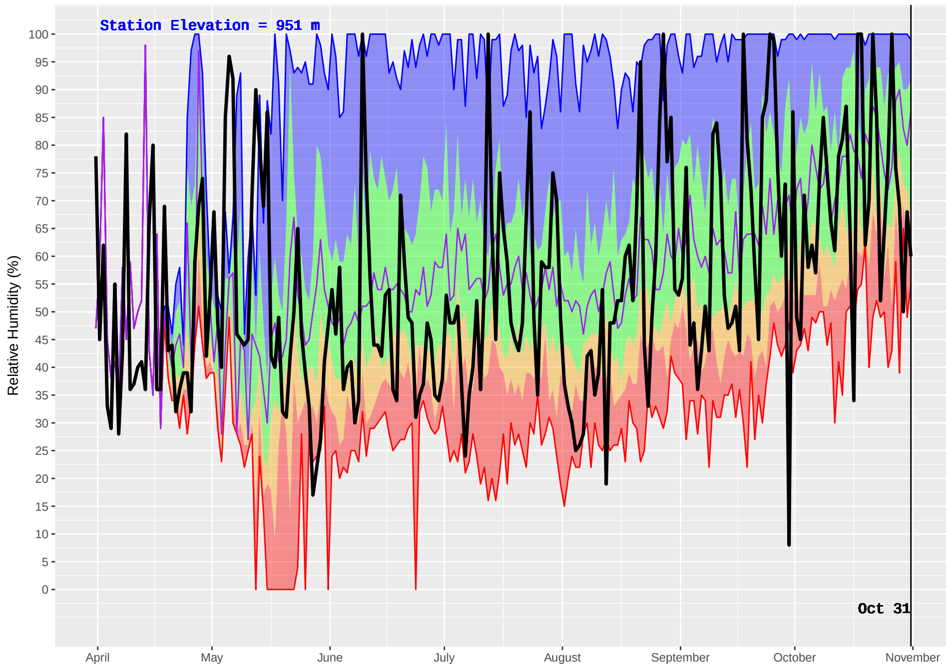
NORTH BABINE (173) : Historical (1986–2016) and Current (2017) Noon Relative Humidity
